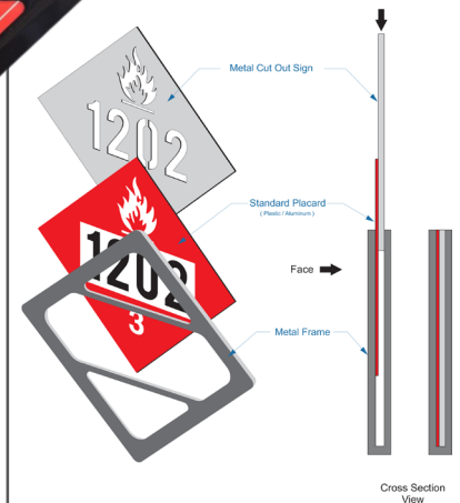
Placard Assembly
